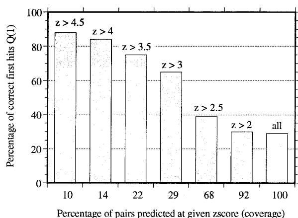
Figure 3. Focusing on stronger predictions. The percentage of correct first hits can be increased by focusing on hits detected with higher z-scores. However, the increase of accuracy was at the expense of coverage. For example, at z > 3.5 75% of all first hits were correct, but only for 22% of all test proteins did the first hit reach a z-score > 3.5 . In other words, a fifth of the test cases predicted most strongly reached an accuracy of 75% ( Q(1) ).
